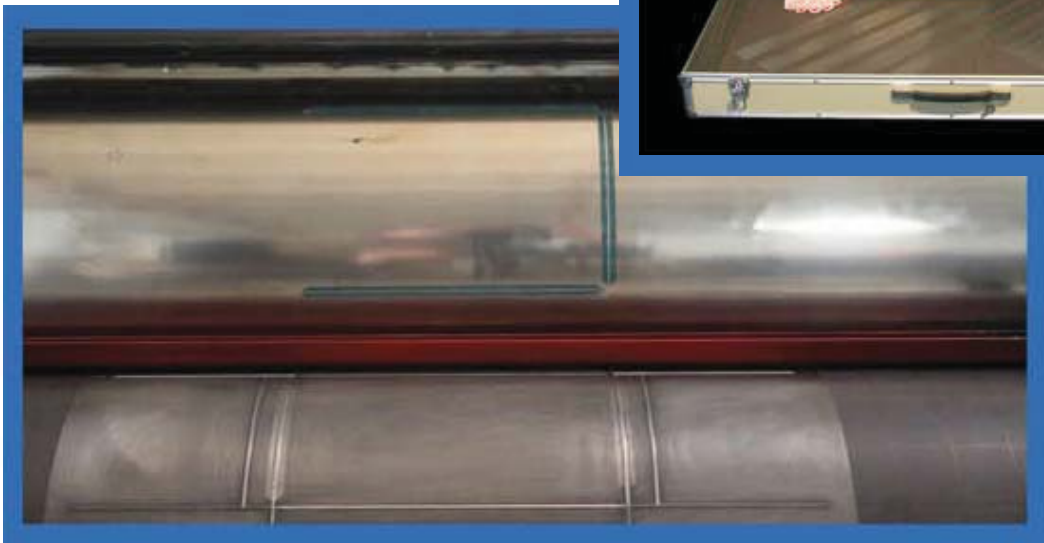
Flexible Cutting and Creasing Die is shown mounted on the MAG-base with the corresponding Female Matrix for Creasing shown on the Super-Care Impression Cylinder Jacket
